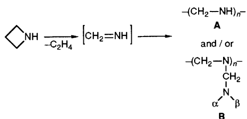
Scheme 2 In B, \alpha, \beta indicate H, \text{CH}_2\text{NH}_2 , or \text{CH}_2\text{N}(\text{CH}_2\text{N} < )_2
