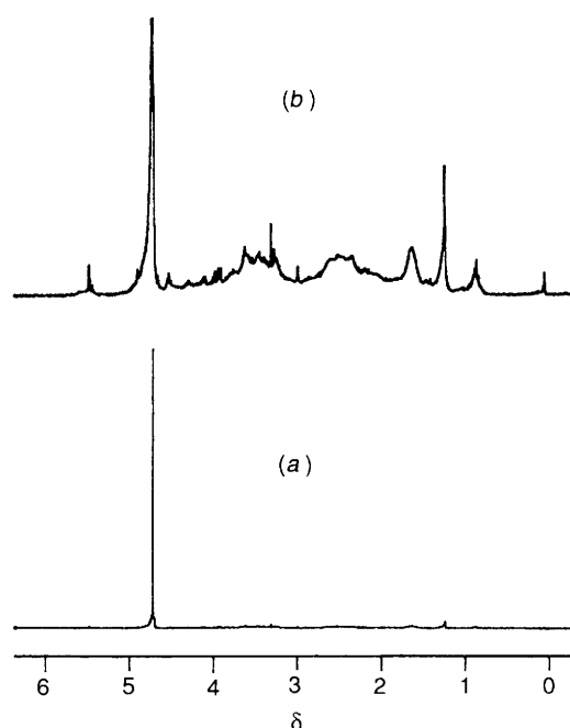
Fig. 1 Standard (a) and amplified (b) 400.13 MHz 1 H NMR spectrum of the deposit in CDCl 3 at 300 K
