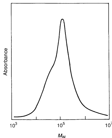
Fig. 2 Elution profile of the deposit from gel permeation chromatography
